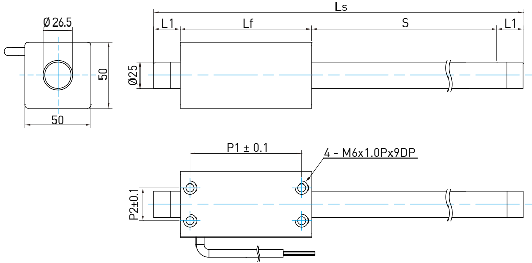
■ Dimensions of LMTB forcers and stators
