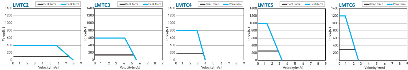
■ Force and velocity curve( DC bus voltage = 325 V DC )
