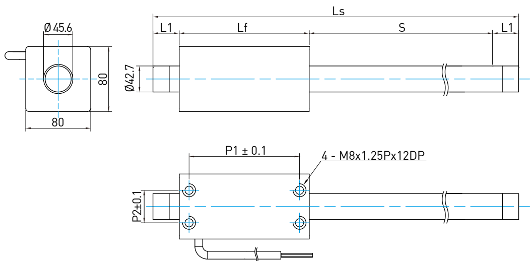
■ Dimensions of LMTD forcers and stators
