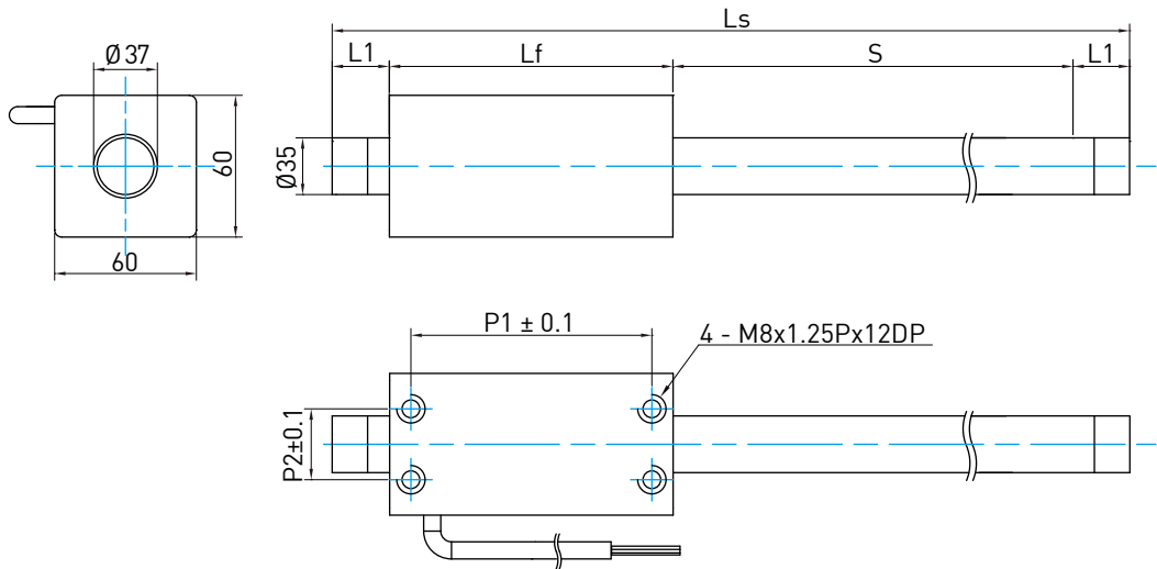
■ Dimensions of LMTC forcers and stators
