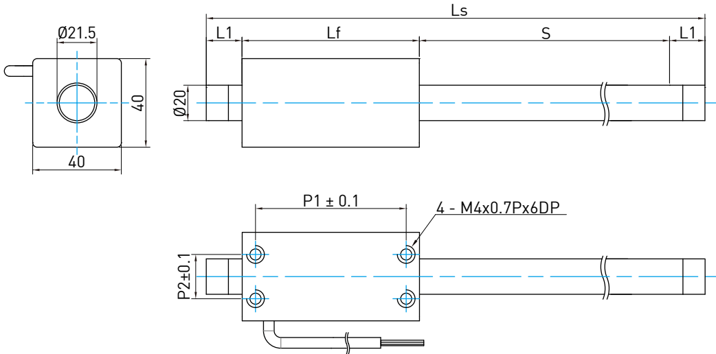
■ Dimensions of LMTA forcers and stators
