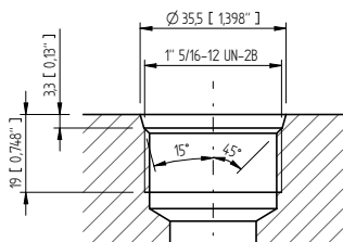
Pressure port Type "U"
